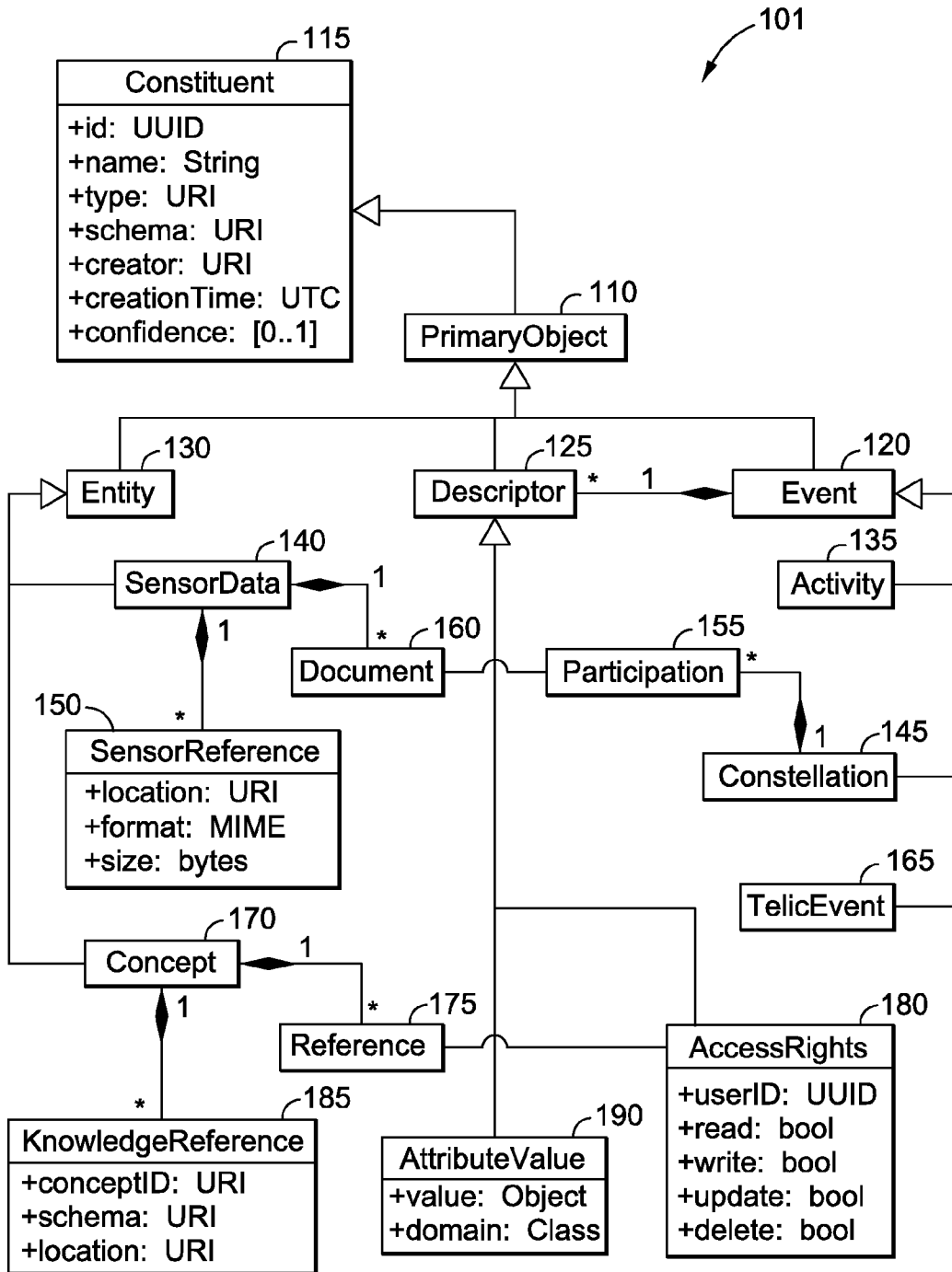
UML CLASS DIAGRAM OF THE GENERIC EVENT MODEL
